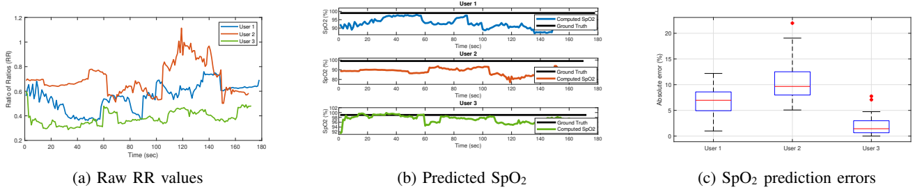
Fig. 2: SpO 2 measurements using the ratio-of-ratio (RR) method on three different users exhibiting SpO 2 around 99%. The RR values vary significantly (Fig. 2a) even if the ground truth SpO 2 remains constant throughout the experiment – making linear regression extremely challenging. The result is a significant amount of errors in the predicted SpO 2 values (Fig. 2b, Fig. 2c).
