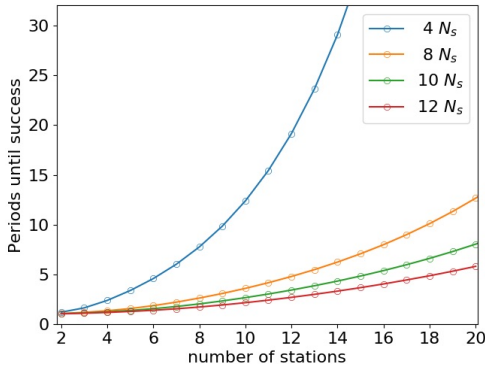
Fig. 10: Increasing the period size leads to succeeding early. However, it also reduces the time reserved for data transmission (DTI) in each beacon interval.
